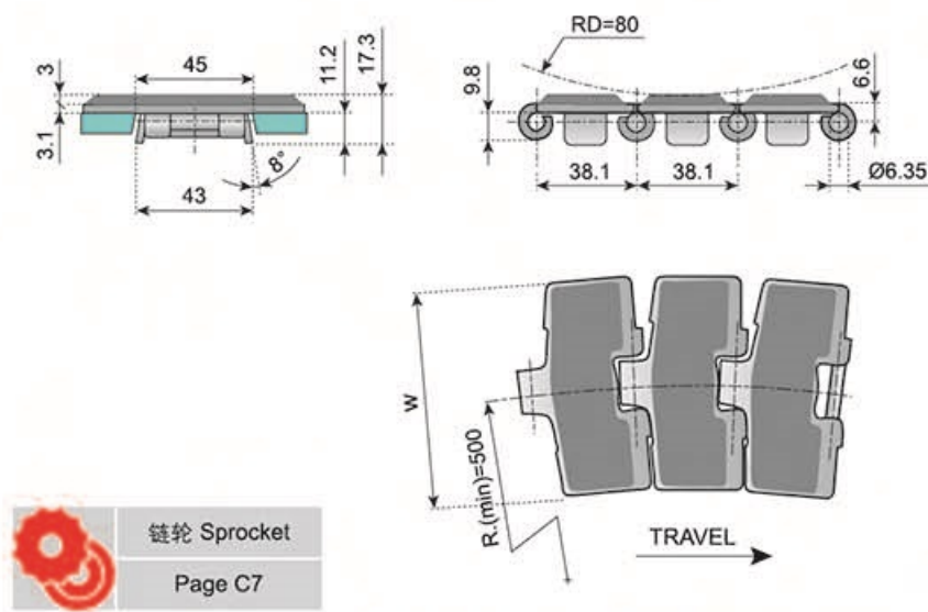
SS881G 防滑侧弯平顶链 SS881G WITH RUBBER TOP
