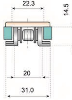
1843 扣链式转弯输送链 1843 SIDEFLEXING PLASTIC CHAINS with base roller chains 12.7mm(1/2")pitch
