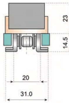
1843G3 扣链式转弯输送链 1843G3 SIDEFLEXING PLASTIC CHAINS with base roller chains 12.7mm(1/2")pitch
