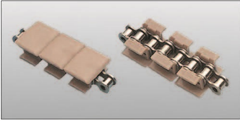
1843 扣链式转弯输送链 1843 SIDEFLEXING PLASTIC CHAINS with base roller chains 12.7mm(1/2")pitch
