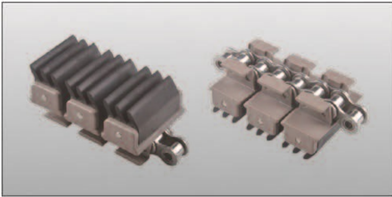
1843G3 扣链式转弯输送链 1843G3 SIDEFLEXING PLASTIC CHAINS with base roller chains 12.7mm(1/2")pitch
